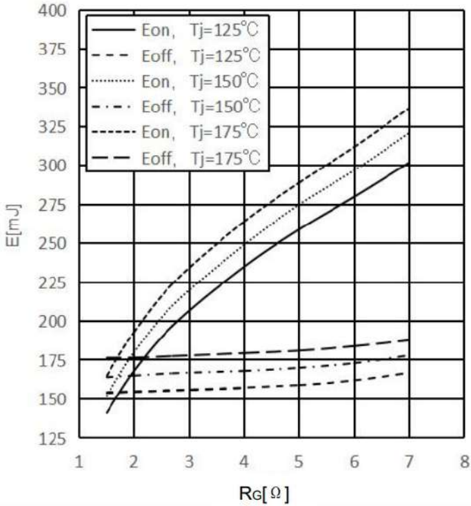
Switching losses IGBT, Inverter (Typical), Inclusive R_{CC}+E_{E'} E = f(R_G) V_{GE} = +15V/-8V, I_C = 450A, V_{CE} = 900V
