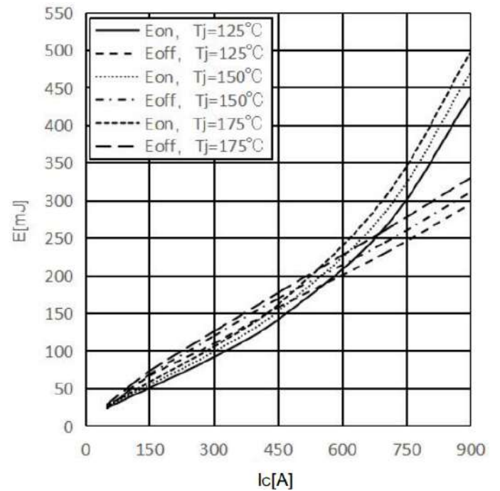
Switching losses IGBT, Inverter (Typical), Inclusive RCC+EE' E = f(I_c)
