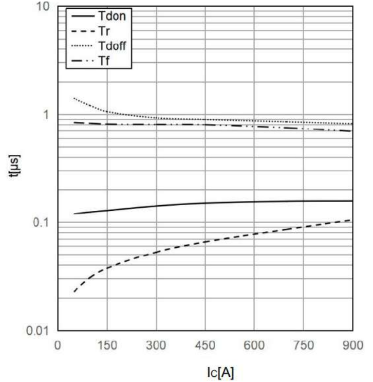
Switching times IGBT, Inverter (typical) IGBT t_{don} = f(I_C), t_r = f(I_C), V_{GE} = +15V/-8V, V_{CE} = 900V R_{gon} = 1.5\Omega, R_{Goff} = 5\Omega, T_j = 175^\circ C
