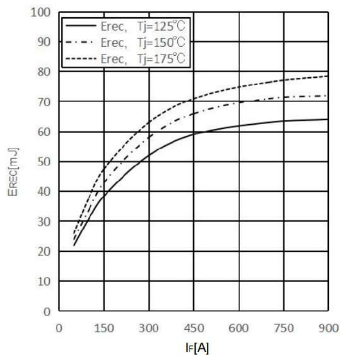
Switching Losses FRD, Inverter (typical), Inclusive R_{CC} + EE' E_{rec} = f(I_F), R_{Gon} = 1.5\Omega, V_{CE} = 900V
