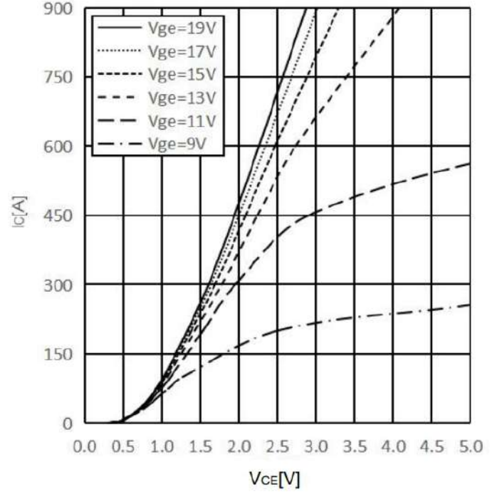
Output characteristic IGBT, Inverter (typical), Inclusive RCC+EE' I_c = f(V_{CE}), T_{vj} = 175^\circ C
