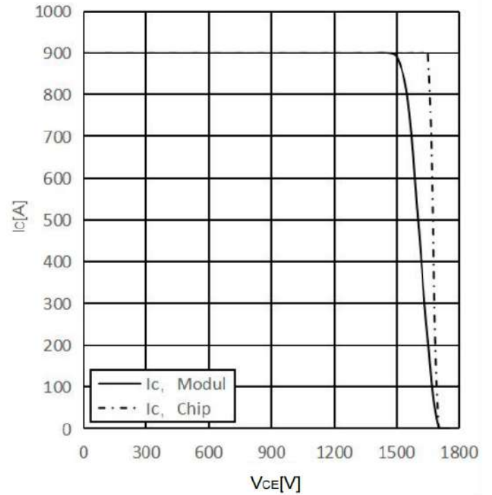
Reverse bias safe operating area IGBT, Inverter(RBSOA) I_c = f(V_{CE}) V_{GE} = +15V/-8V, R_{goff} = 5\Omega, T_{vj} = 175^\circ C
